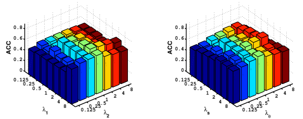
Fig. 10. Sensitivity analysis. Classification accuracy on varying regularization parameters \lambda_1 and \lambda_2 when \lambda_s and \lambda_\theta are fixed (left); \lambda_s and \lambda_\theta with \lambda_1 and \lambda_2 fixed (right).
